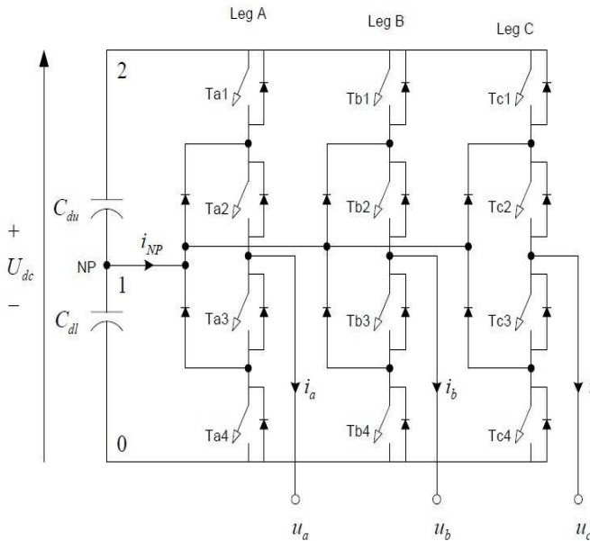
Fig.1 NPC converter topology
