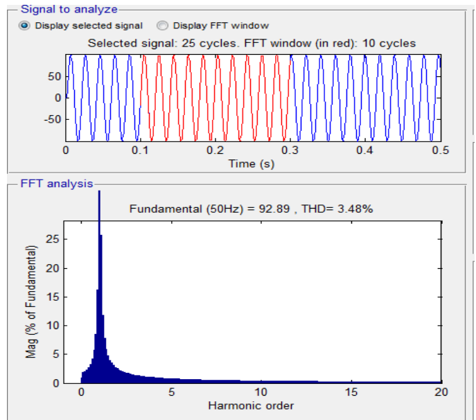
Fig. 9 Harmonic elimination of FFT analysis
