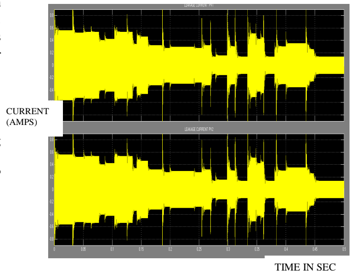
Fig.10Elimination of leakage current in PV panel
