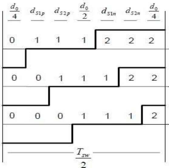
Fig.6 Switching pattern for three-medium vector modulation
