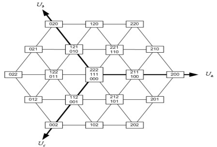
Fig.5 Space vector diagram for a three-level converter
